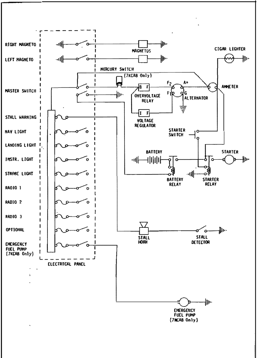
FIGURE 6-4 ELECTRICAL SYSTEM SCHEMATIC
