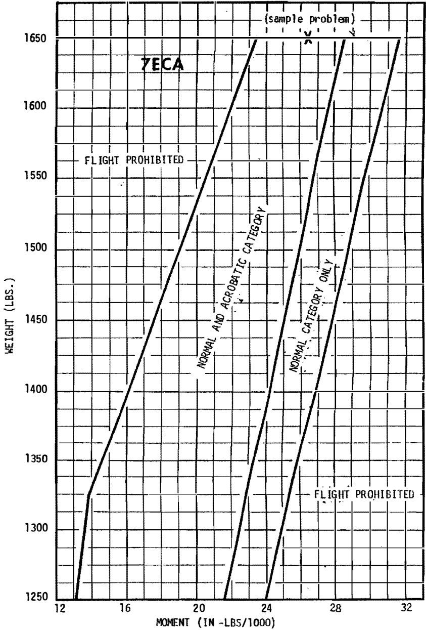
FIGURE 5-3 FLIGHT ENVELOPE - 7ECA ONLY
