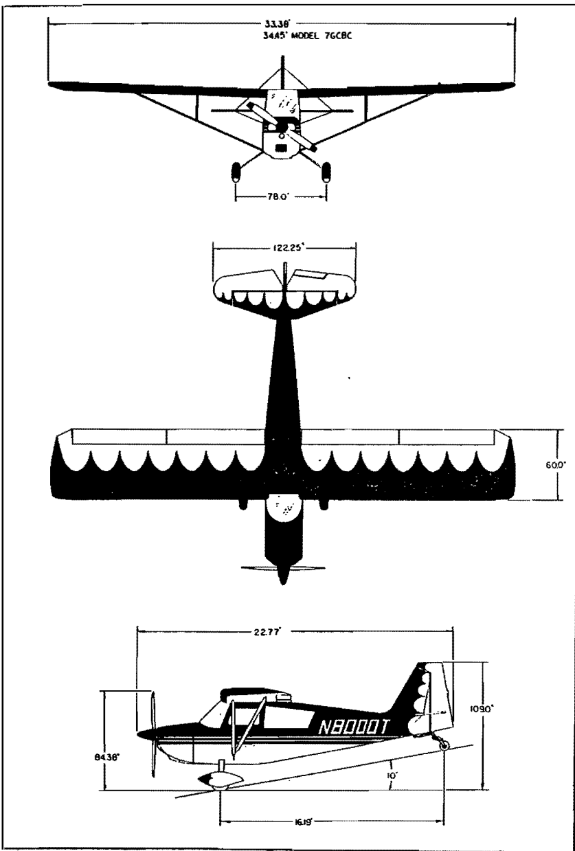
FIGURE 6-2 CITABRIA THREE-VIEW
