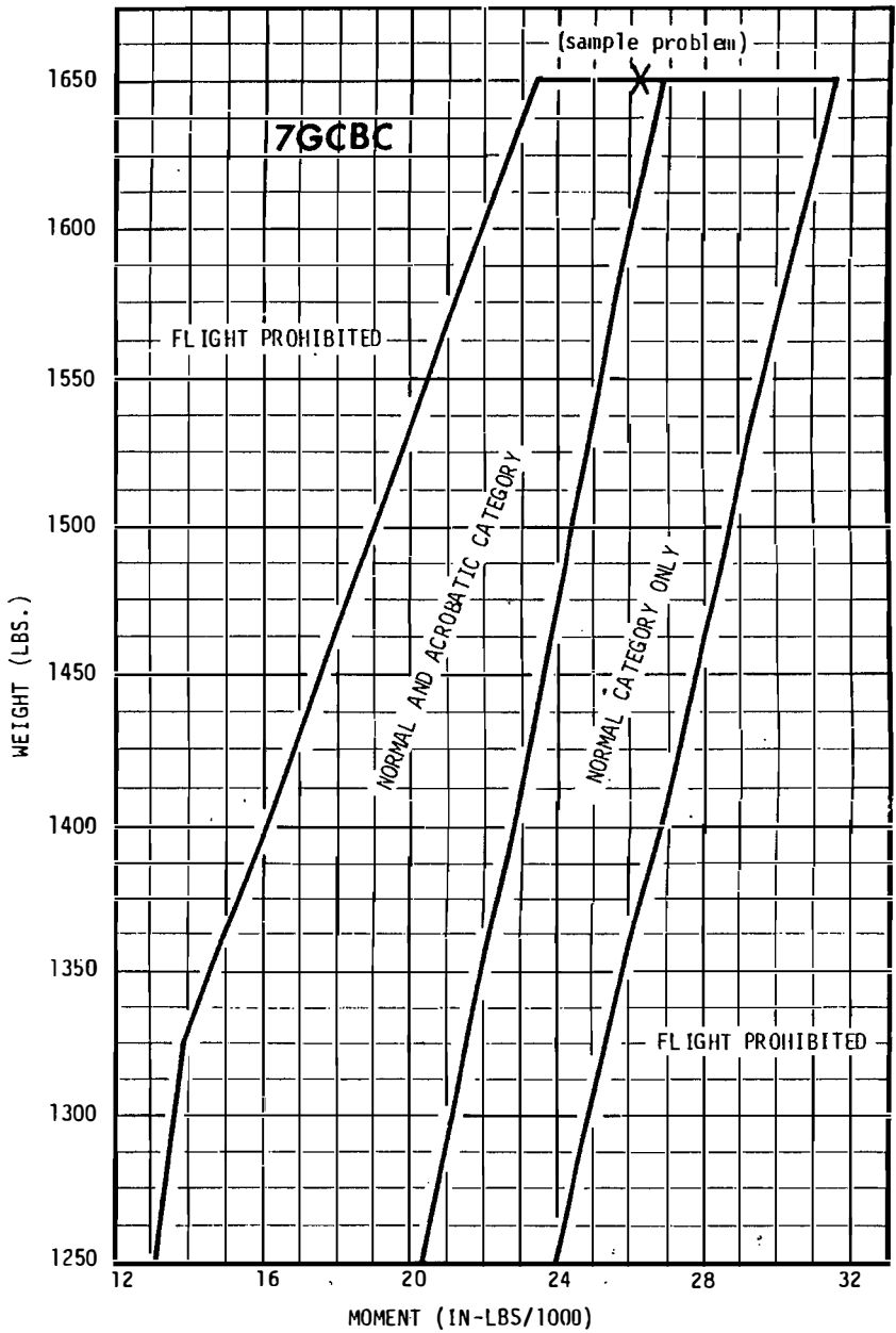
FIGURE 5-5 FLIGHT ENVELOPE - 7GCBC ONLY
